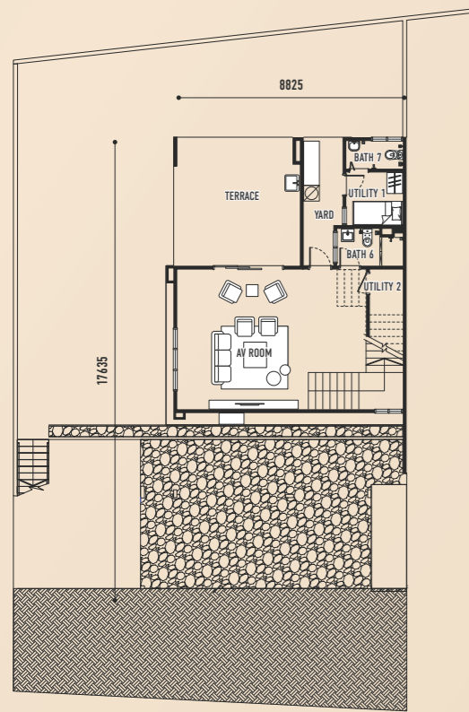
LOWER GROUND
